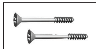
yy. Tornillos Ø 3/16" x 1 5/8" (Ø 4 mm x 42 mm)* x 2
