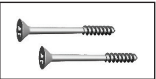
yy. Screws \varnothing 3/16" x 1 5/8" ( \varnothing 4 mm x 42 mm)* x 2
