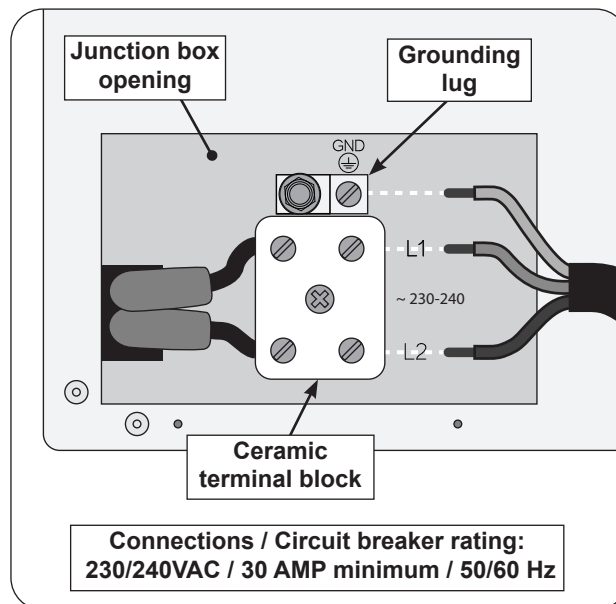
Fig. 28-2 Wire connection diagram
