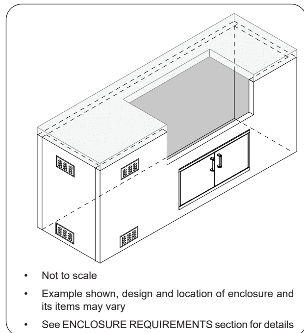
Fig. 27-1 Enclosure construction overview
