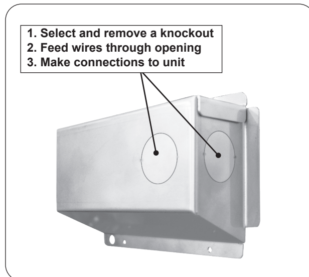
Fig. 28-1 Junction box knockouts
