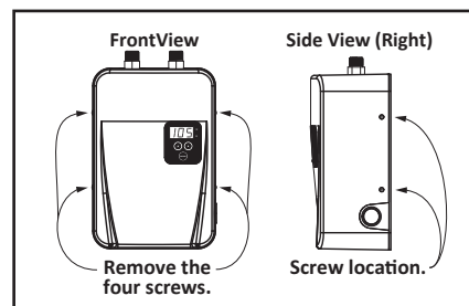
Figure 5 - Removing the front cover.
