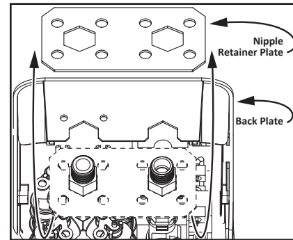
Figure 44 - Nipple retainer plate removal.
