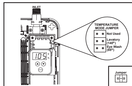
Figure 6 - Temperature mode jumper.
