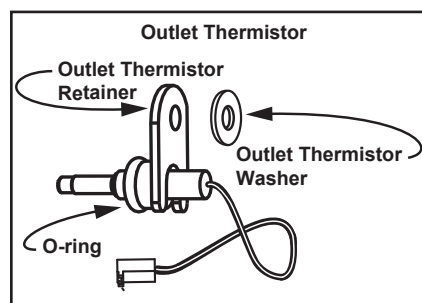
Figure 24 - Outlet thermistor with o-ring..
