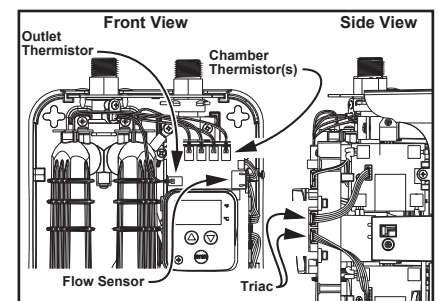
Figure 46 - Control Board Component Connections
