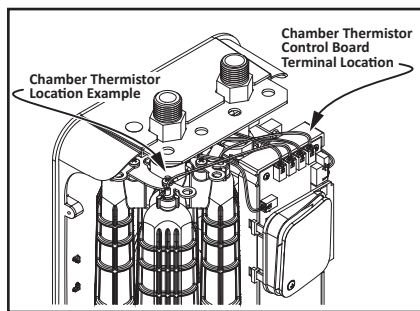
Figure 25 - Chamber thermistor location.
