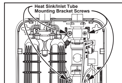
Figure 43 - Heat-sink/inlet tube mounting bracket screws.
