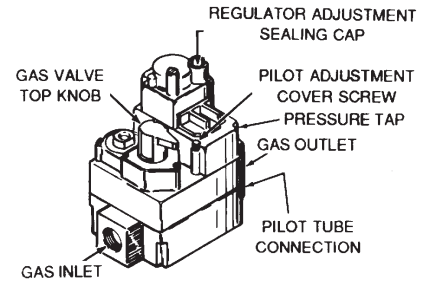
WHITE-RODGERS GAS VALVE LP VALVE
