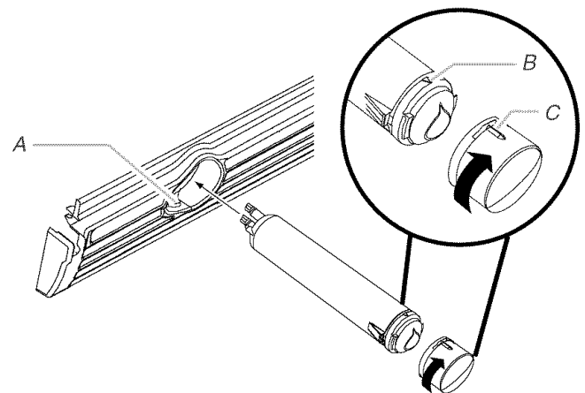
A. Eject button B. Groove on filter C. Ridge on cap
