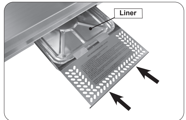
Fig. 32-3 Install drip tray
