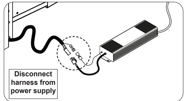
Fig. 28-2 Disconnect harness
