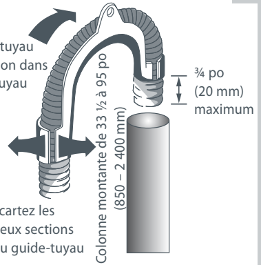
Fig.3 Installation du guide-tuyau
