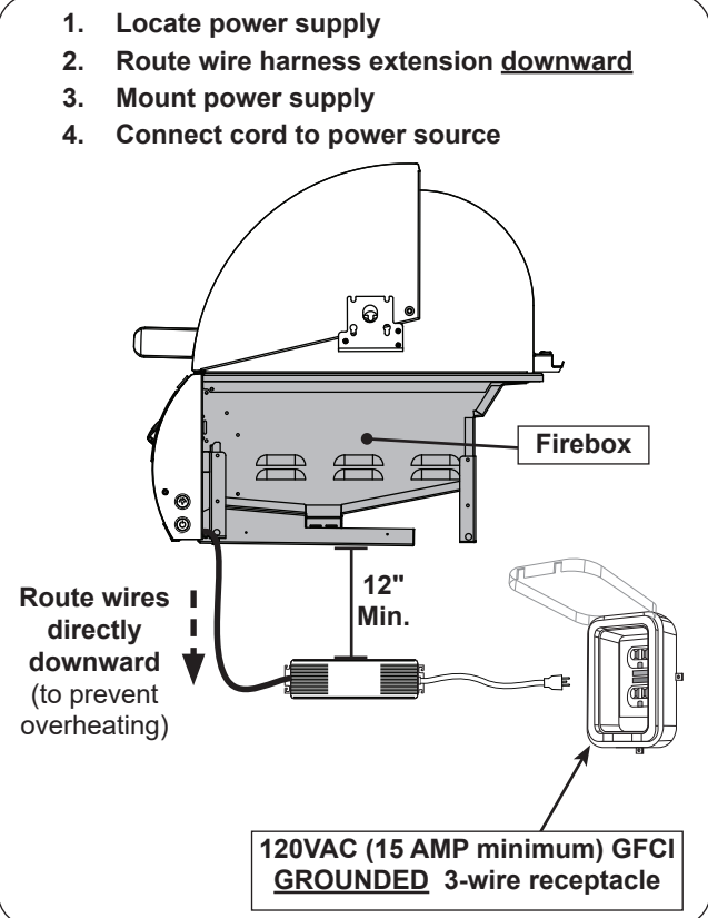
Fig. 30-3 Electrical installation
