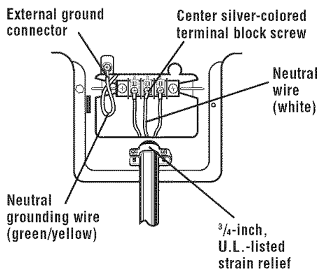
3-Wire Connection with Frame-Grounding Conductor
