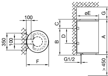
Fig. 1: Vertical installation on a wall
