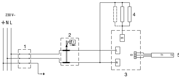
Fig. 6: Electric installation
