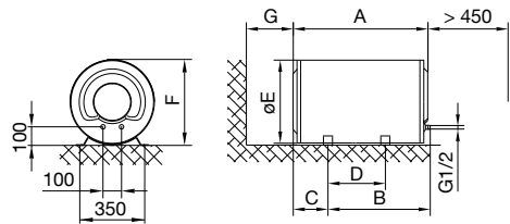
Fig. 2: Horizontal installation on the floor
