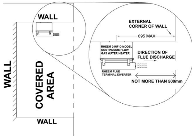
24NF-D model with a Flue Terminal Diverter installed in compliance with AS/NZS 5601.1
