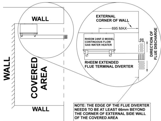
24NF-D with an Extended Flue Terminal Diverter installed in compliance with AS 5601 and AS/NZS 5601.1
