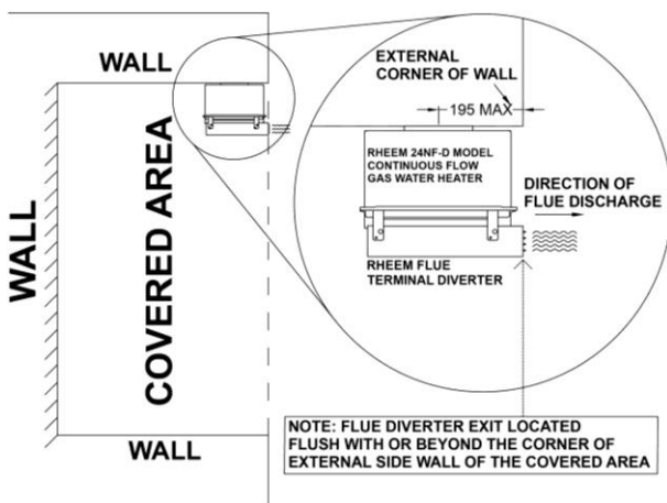
24NF-D with a Flue Terminal Diverter installed in compliance with AS 5601 and AS/NZS 5601.1
