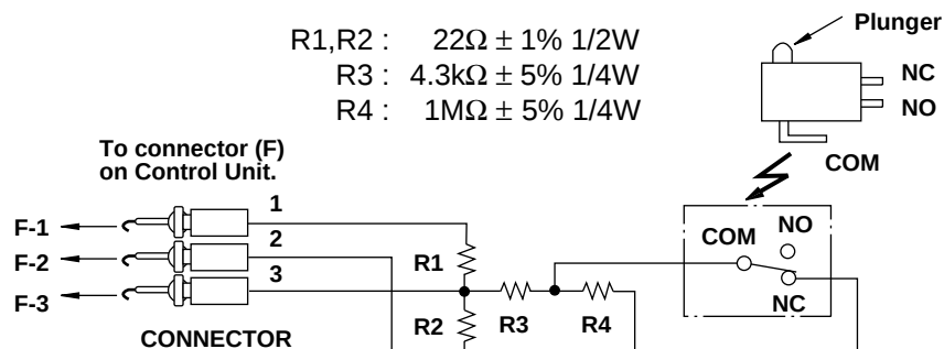
Sensor Dummy Resistor Circuit
