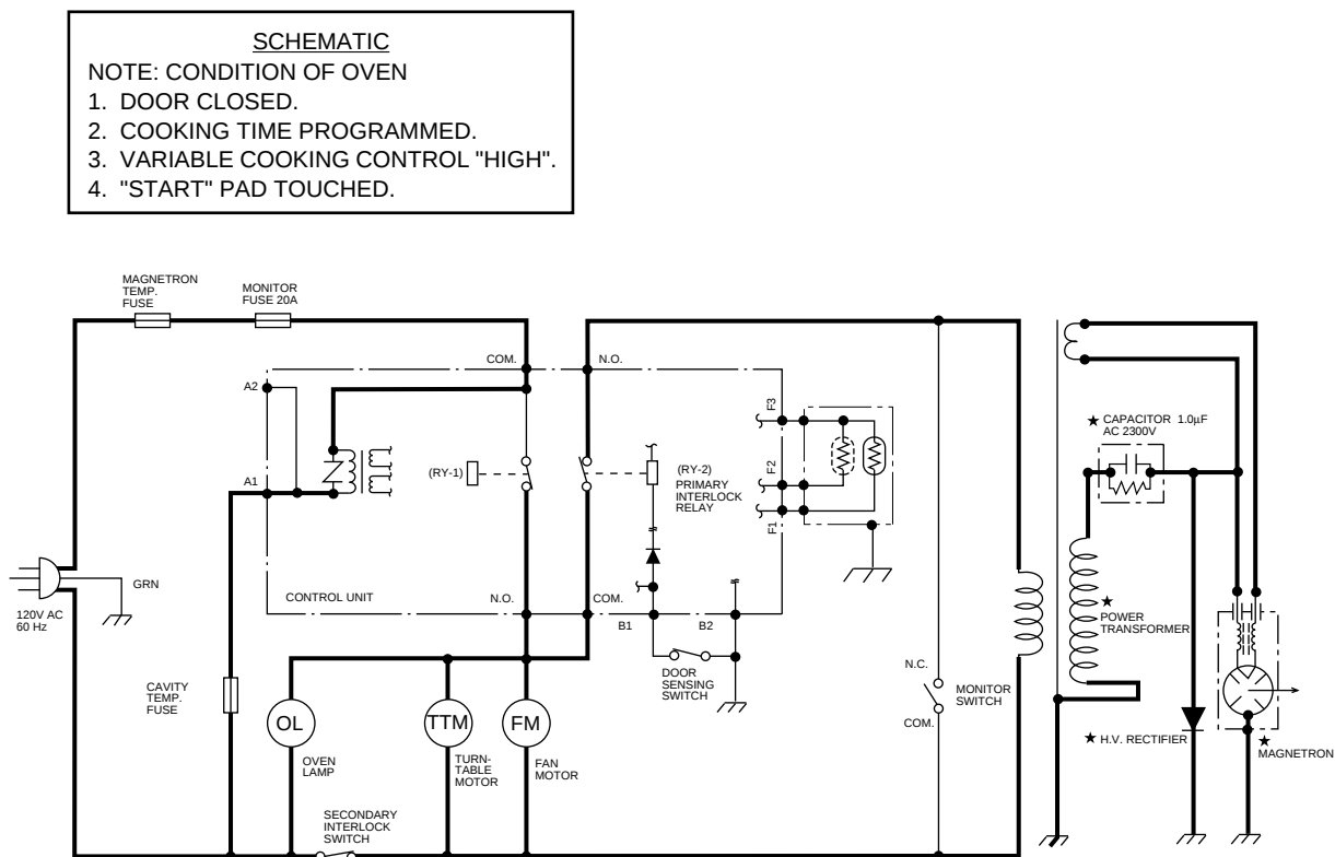
Figure O-1. Oven Schematic-Off Condition
