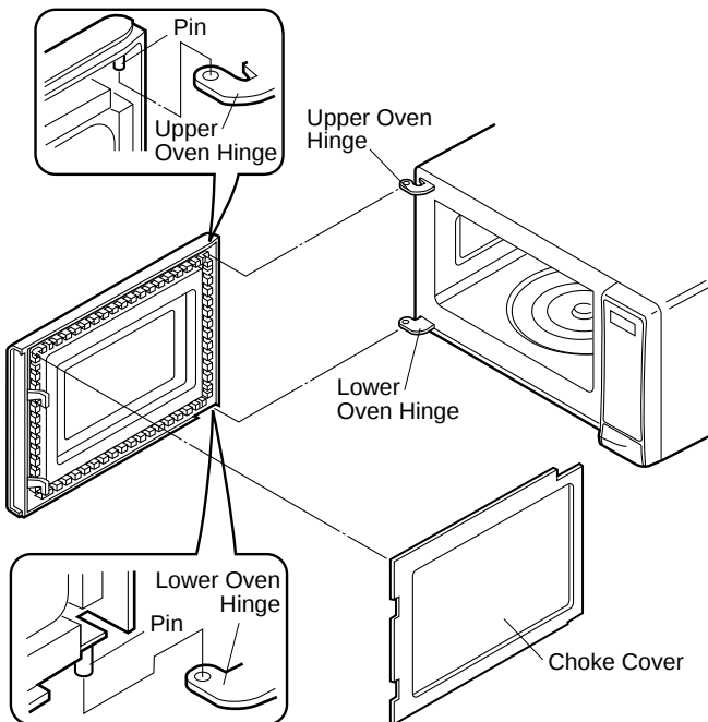
Figure C-5. Door Replacement
