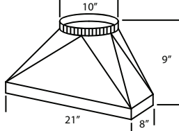
M1200 STANDARD TRANSITION
