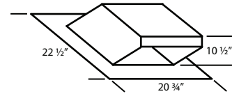
LOW PROFILE ROOF JACK (MAXIMUM 4/12 PITCH)
