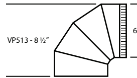
ADJUSTABLE ELBOW
