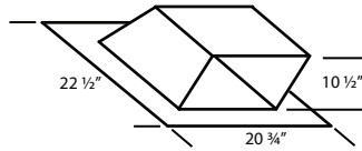
LOW PROFILE ROOF JACK (MINIMUM 4/12 PITCH)
