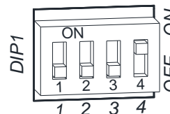
dip switch settings without temperature controller
