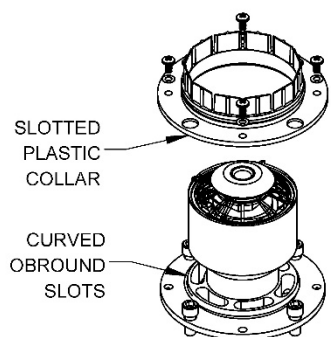
MFI (FLAKER) HEAD ASSEMBLY
