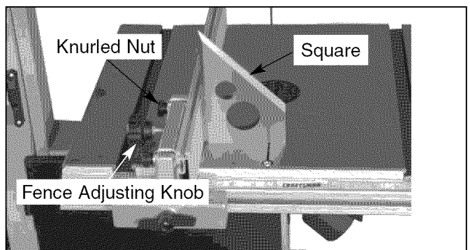
Figure 28 - Fence Adjustment
