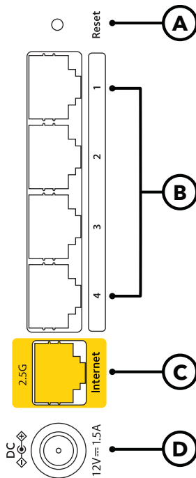
Figure 3. Rear panel
