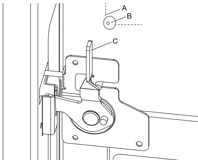
Figure 1: Latch
