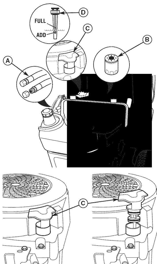
Figure 25. Oil Change - Kohler Models
