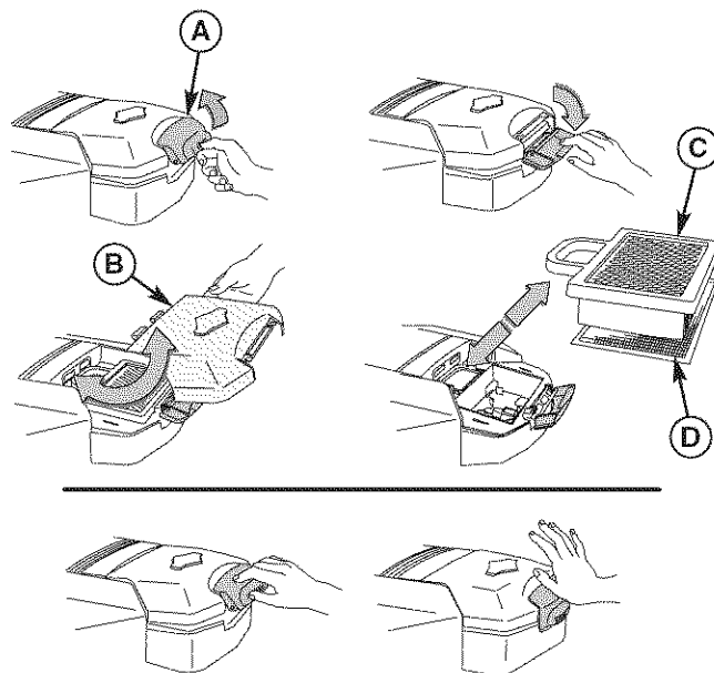
Figure 30. Air Filter Assembly - Briggs & Stratton Models
