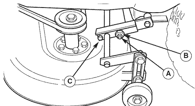
Figure 39. Side-to-Side Adjustment
