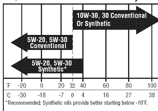
Figure 24. Recommended Engine Oil - Kohler Models
