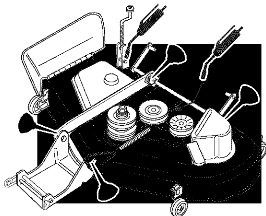
Figure 16. Mower Lubrication
