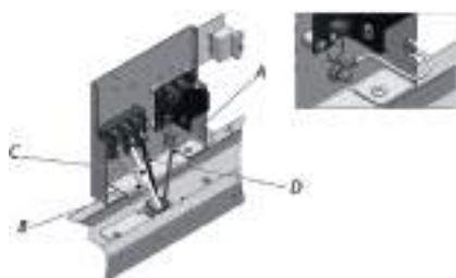
(type B) 4-WIRE CONNECTION
