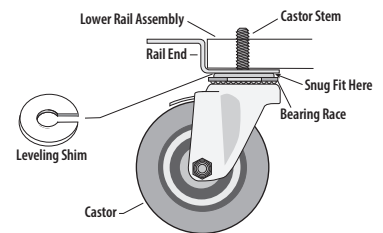
Fig. 7. Install shim(s).
