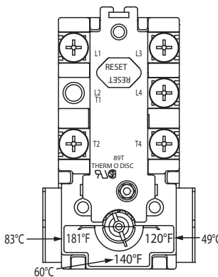
Figure 3. A-8 Thermostat
