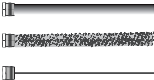
Figure 5. Anode Depletion
