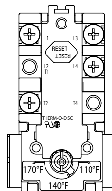
Figure 4. C-2 Thermostat
