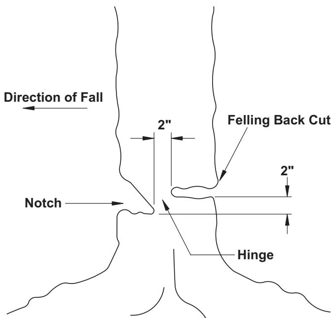
Figure K: Undercutting
