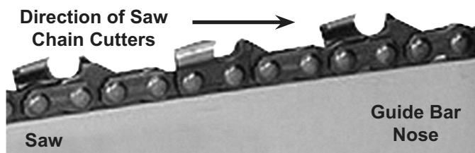
Figure E: Saw Chain Orientation
