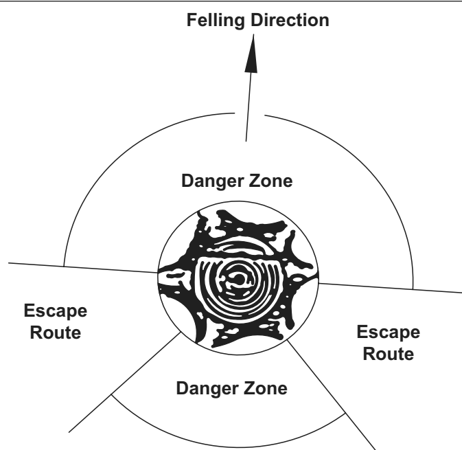
Figure J: Escape Routes
