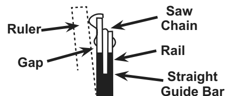
Figure S: Normal Guide Bar
