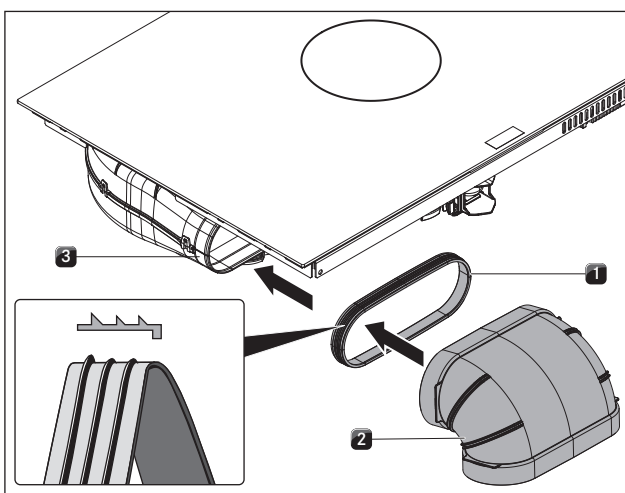
Fig. 6.23 Connecting the duct system
