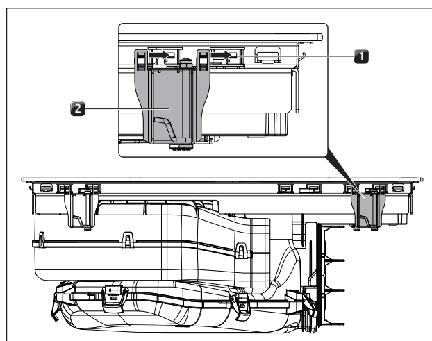
Fig. 6.33 Fitting the installation clamps
