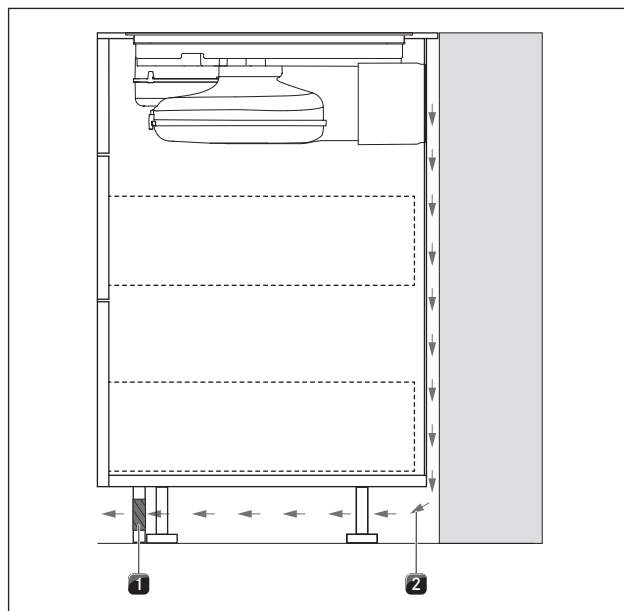
Fig. 6.24 Return flow aperture in the plinth area
