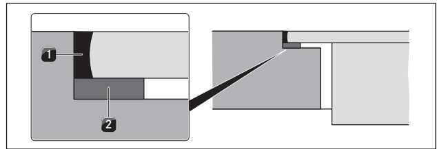
Fig. 6.17 Sealing tape in the case of flush installation
