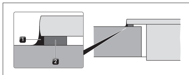
Fig. 6.31 Sealing tape in the case of surface mounting
