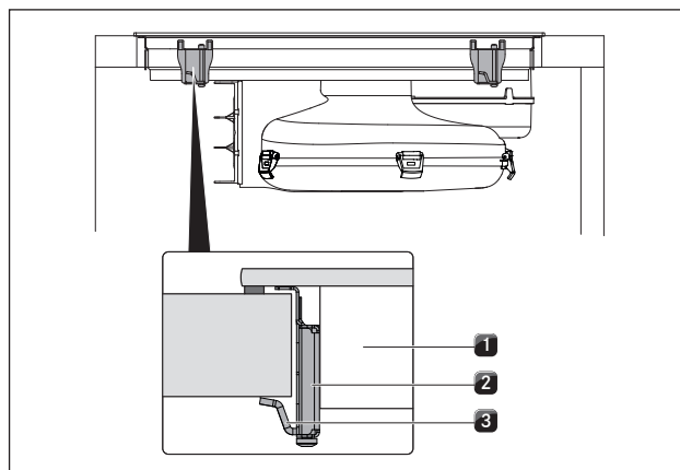
Fig. 6.39 Securing the cooktop
