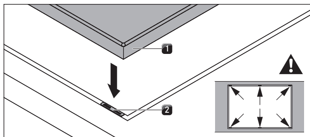
Fig. 6.37 Height adjustment plates
