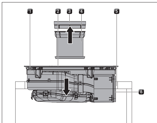
Fig. 6.36 Positioning the cooktop in the centre
