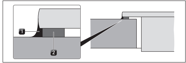
Fig. 6.16 Sealing tape in the case of surface mounting
