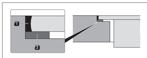
Fig. 6.32 Sealing tape in the case of flush installation
