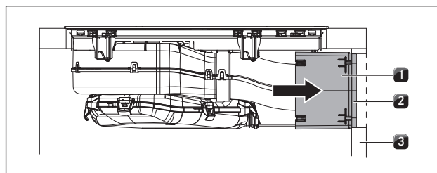
Fig. 6.40 Connection with the back wall
