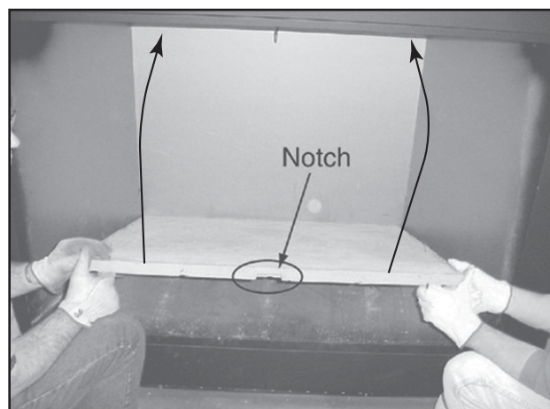
Figure 8.3 Install Back Refractory
