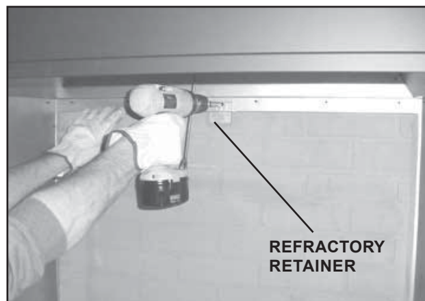
Figure 8.4 Attach Back Refractory
