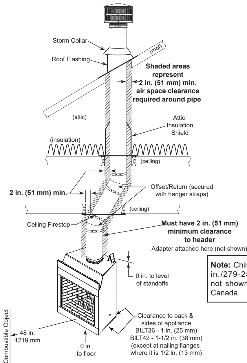
Figure 3.3 Clearances to Combustible Materials
