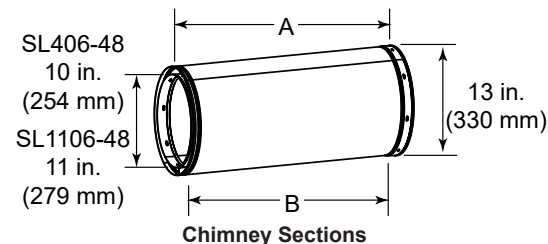
Chimney Sections
