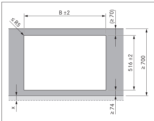
Abb. 5.11 Cut-out dimensions for surface mounting
