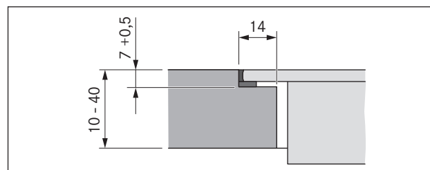
Abb. 5.10 Rebate dimensions for flush installation
