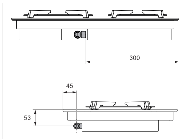
Abb. 5.20 Position of gas connection
