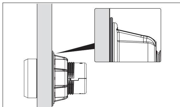
Abb. 5.19 Wave spring when installation is complete
