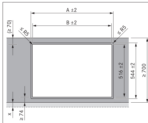
Abb. 5.9 Cut-out dimensions for flush installation
