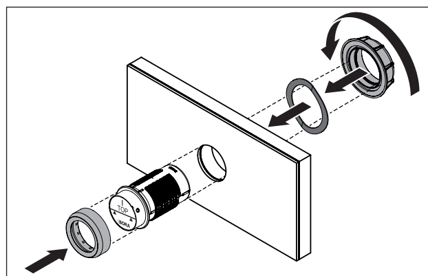
Abb. 5.18 Fitting the control knob
