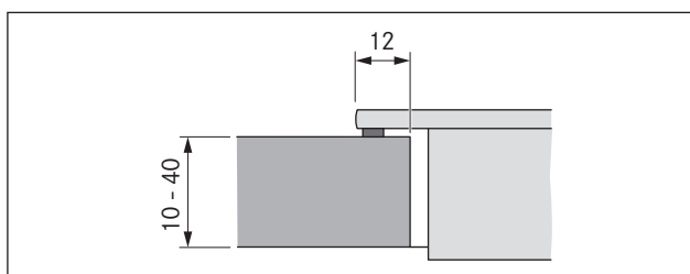
Abb. 5.12 Overlay dimensions for surface mounting
