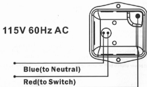
Figure 1: wiring Diagram-Single speed, 120-volt connection.
