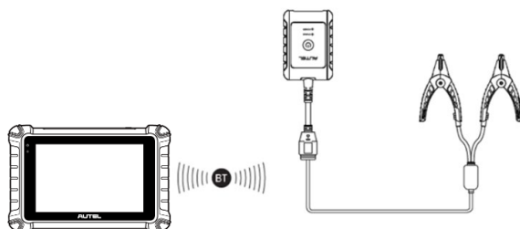
Figure 10-3 Battery Tester Connection Example 1
