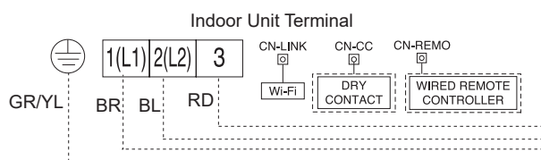
Figure 22: Wired Controller Connection (Example Only).
