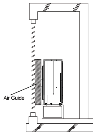
Figure 35: Example of Installing Outdoor Unit Indoors.
