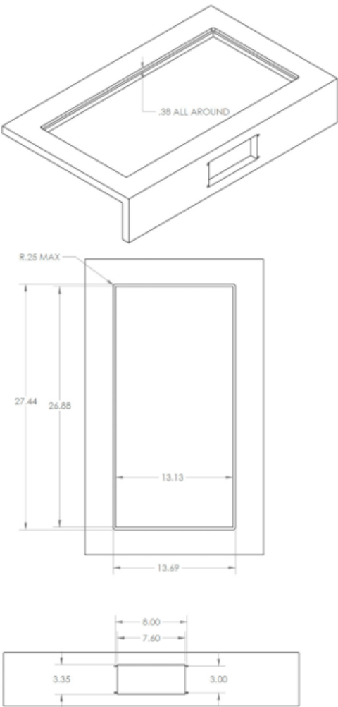
Flush Mount
