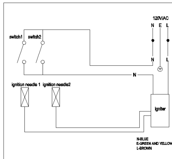
Figure 18(for the appliance with two burners)
