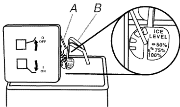
A. Wire shutoff arm B. Ice level adjustment arm
